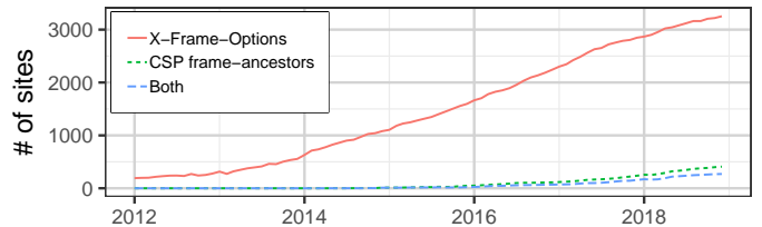
Fig. 9: Evolution of X-Frame-Options and frame-ancestors
